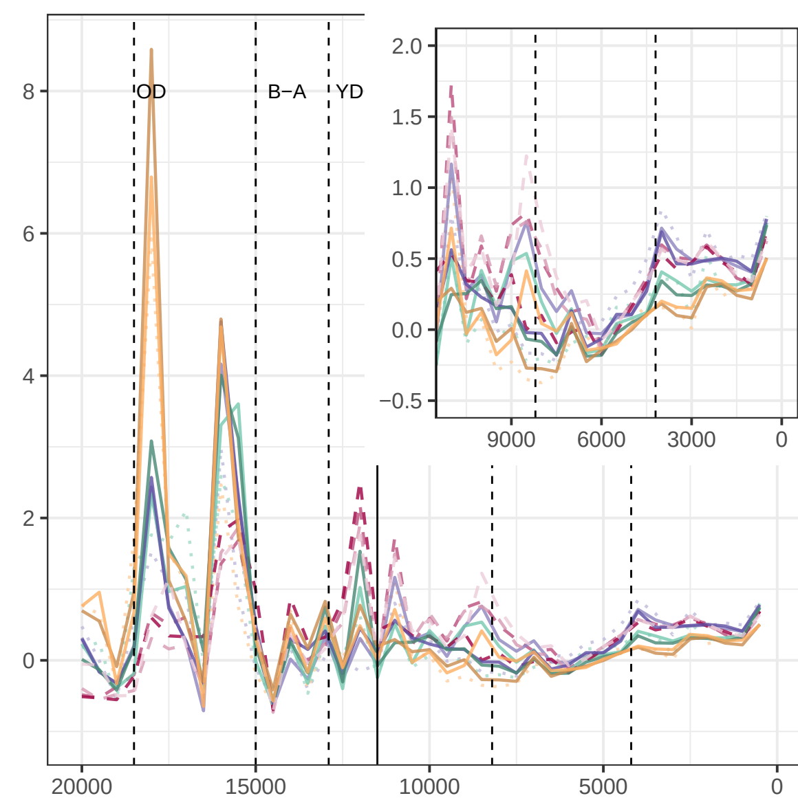
5-fold cross validation results of teh STRK procedure.
