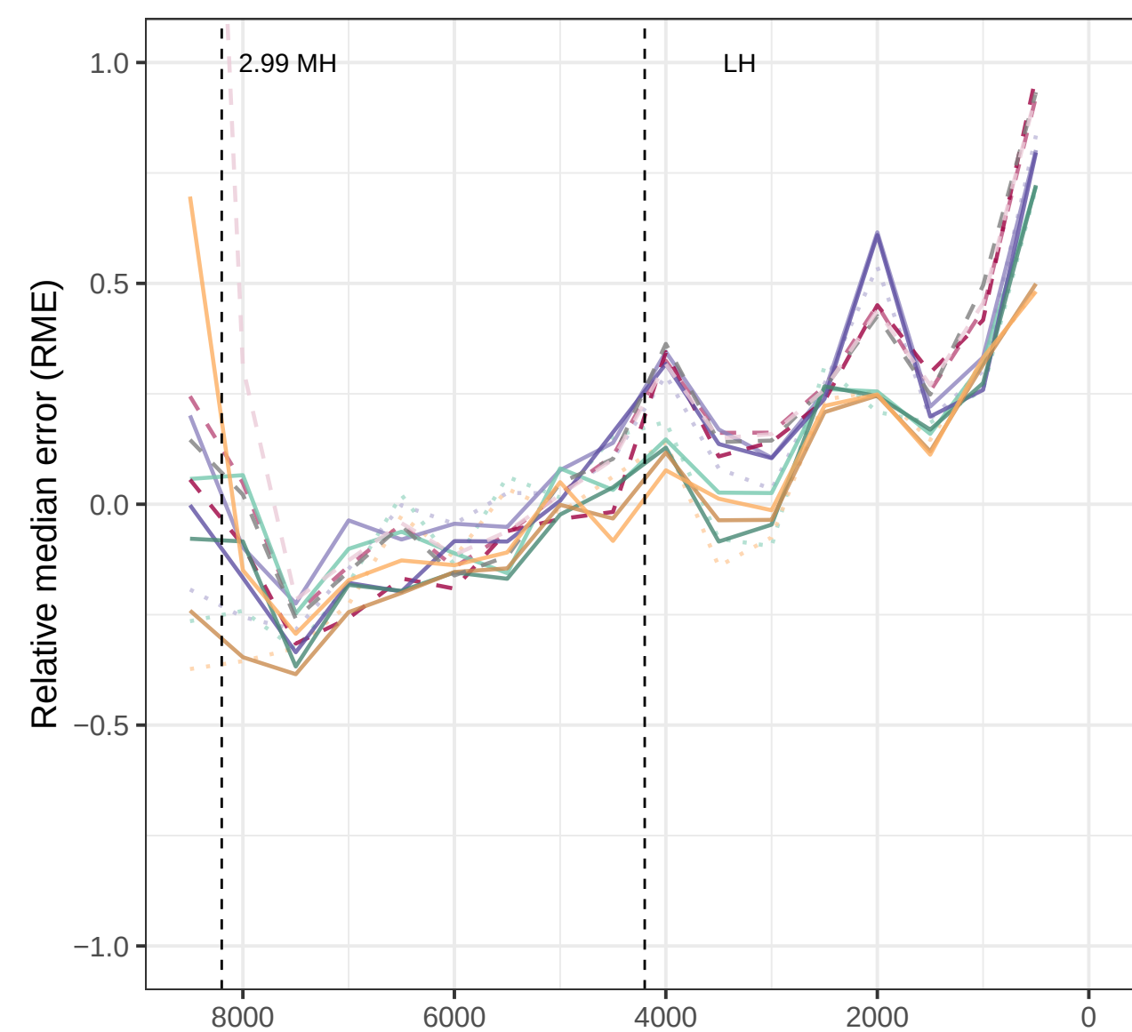
Rolling window results of the STRK procedure.
